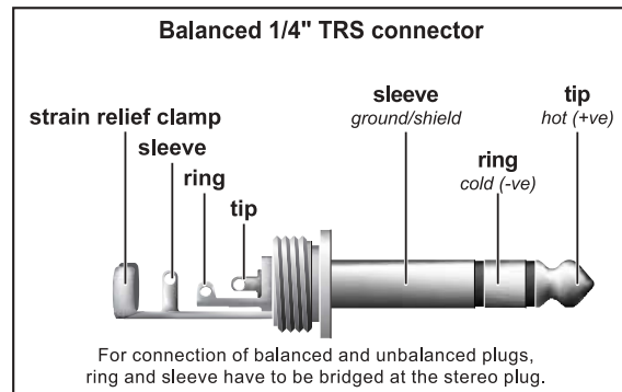
Fig. 4.3: 1/4" stereo plug
